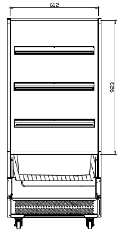
SECTION B-B
