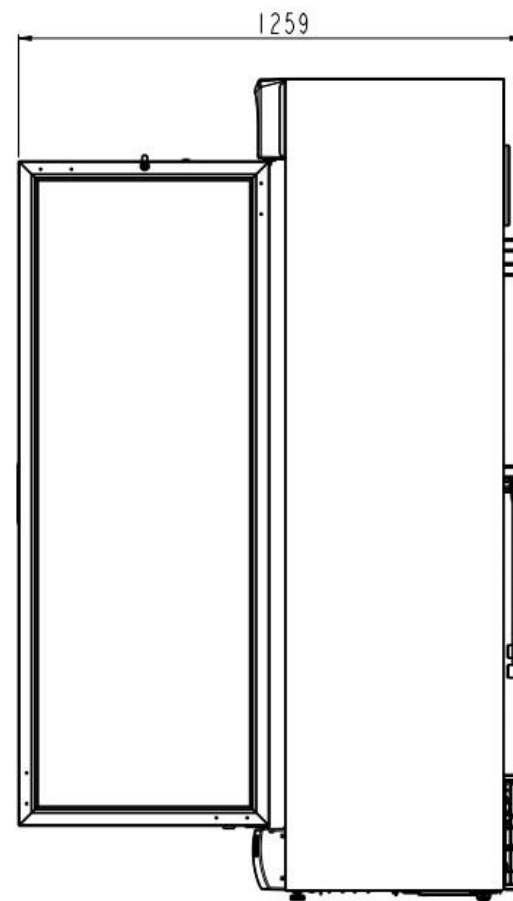
RIGHT
